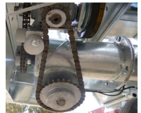
Direct Coupled Chain Drive Augers
